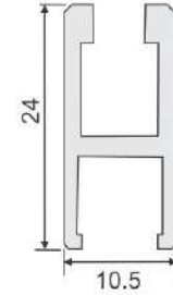
NCST-3 Bottom Frame
