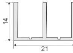
NCST-1 Top Track
